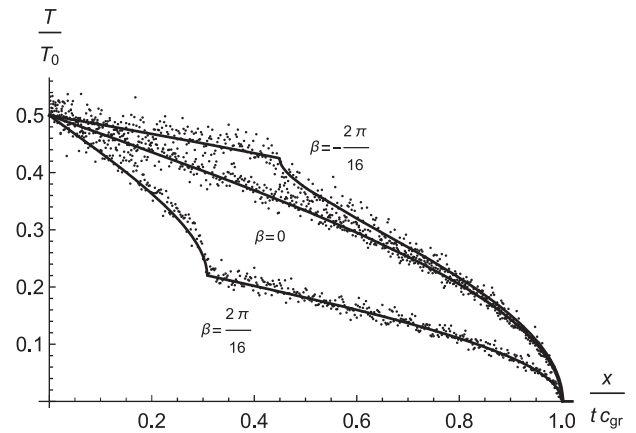
FIGURE 5 Comparison of the heat propagation with the initial perturbation in the form of the Heaviside function for different values of the parameter \beta (solid lines) with the results of the numerical simulation by the particle dynamics method (points)
