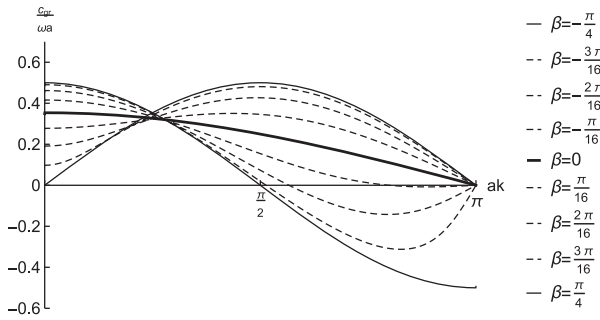
FIGURE 2 Group velocity at different values of the parameter \beta
