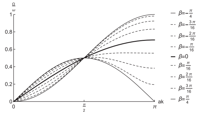
FIGURE 1 Dispersion characteristic of the waves at different values of the parameter \beta
